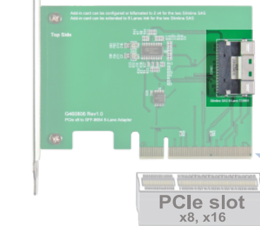
Model No.: PE0804 PCIe x8 to SlimSAS (SFF-8654) 8-Lane Adapter
