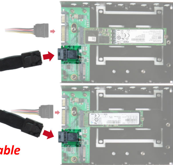
Model No.: PA430G 3.5" Mini SAS HD & SATA to M.2/M.3 NVMe SSD & M.2 SATA Drive Tray
